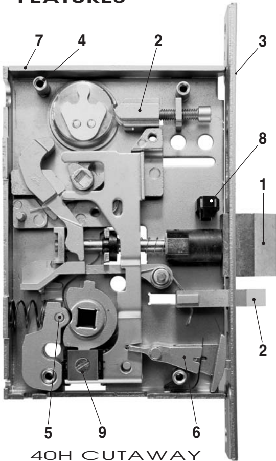
40H CUTAWAY
