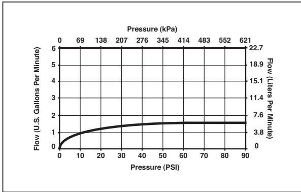
T84101 Body Spray Flow Rate
