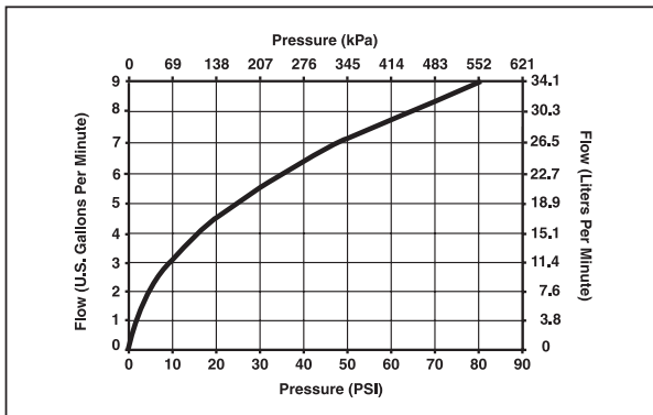
MultiChoice® Medium Flow R60000–UNBX with TempAssure® Thermostatic Cartridge
