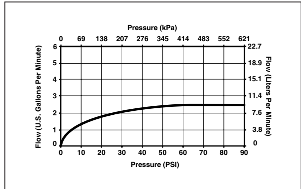
Medium Flow Showerhead Flow Rate
