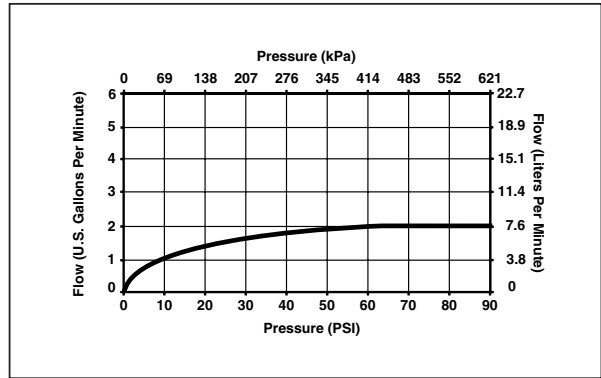
84001 Body Jet and 84110 Body Spray Flow Rate
