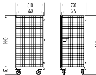
RC/S8 mobile container Illustration shows special equipment
