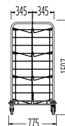
FW-16 - For 16 drinks crates
