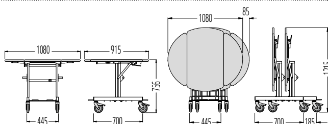
RSVC-Comfort, collapsed
