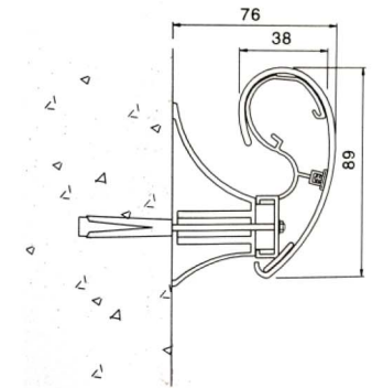
THR89 PVC & Aluminium Mini Handrail in Single color, width: 89mm
